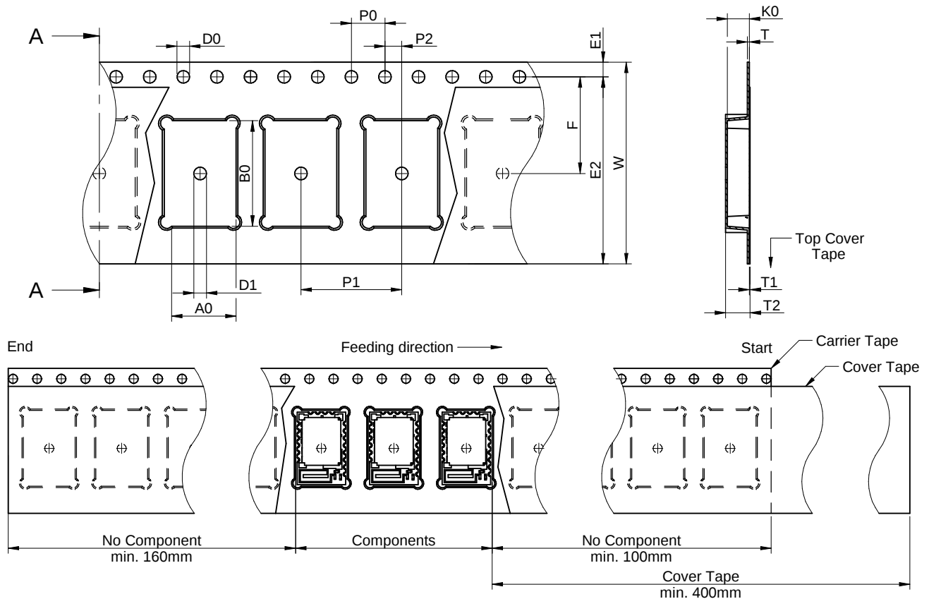
Figure 31: 24 mm Tape
