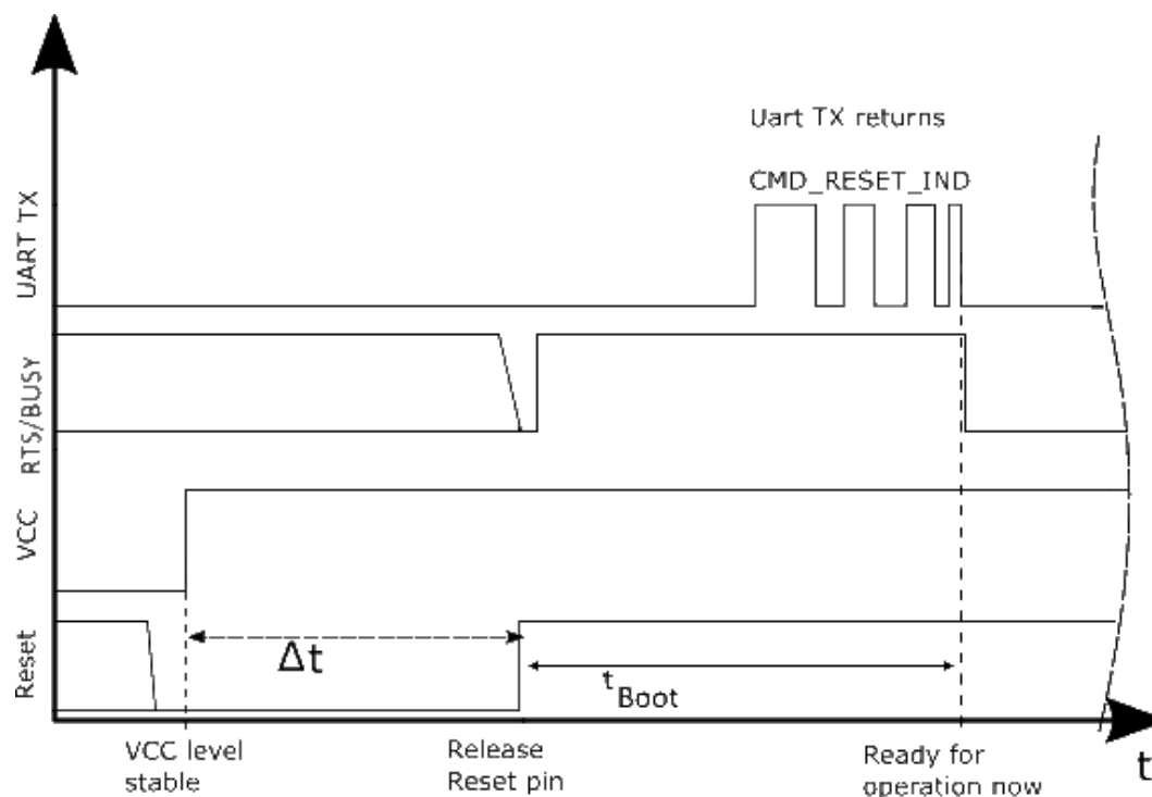
Figure 5: Power up
